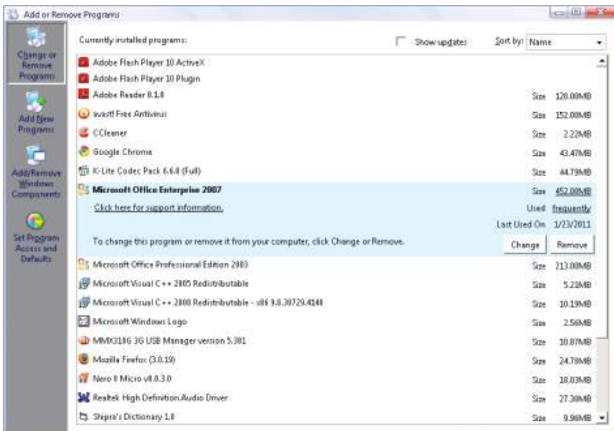
Fig. 3.28: Clicking Remove
