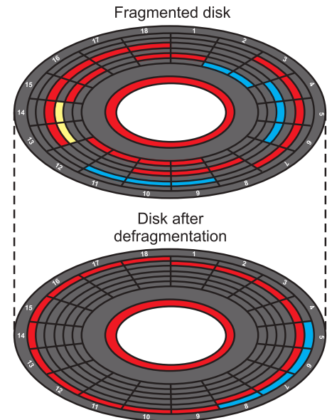
Fig. 3.3: Disk defragmentation
