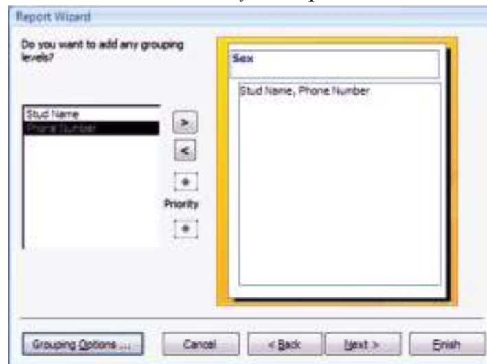
Fig. 2.31: Adding grouping
