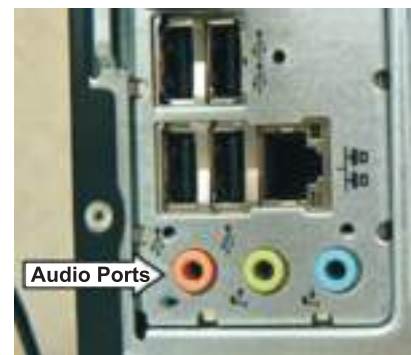
Fig. 3.17: Audio Ports
