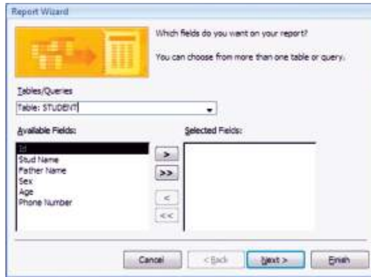
Fig. 2.30: Report Wizard
