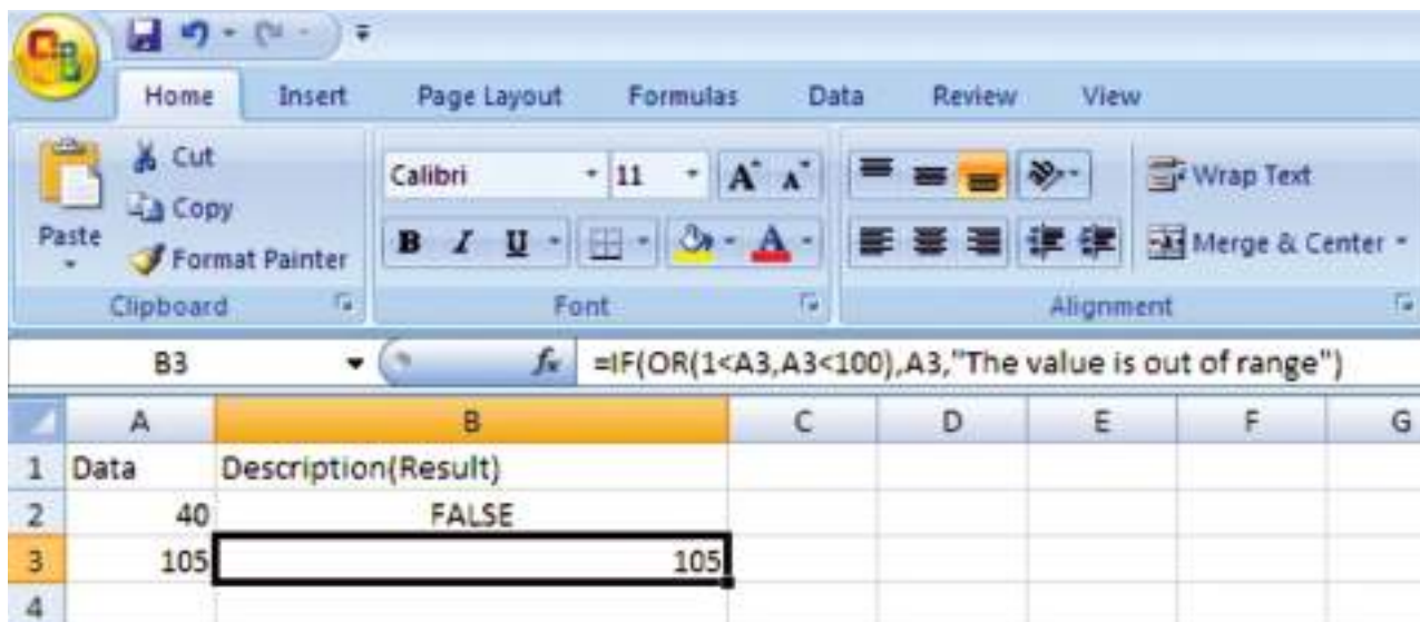
Fig. 2.18: Use of OR
