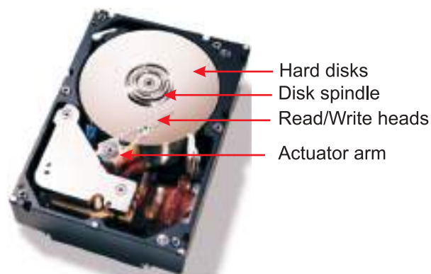
Fig. 3.2: A Hard Disk
